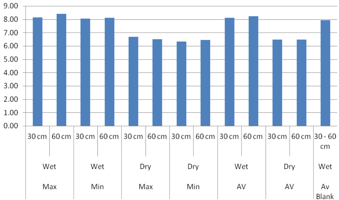
Figure 15: Influence on the pH level under different variations of depth and seasons
