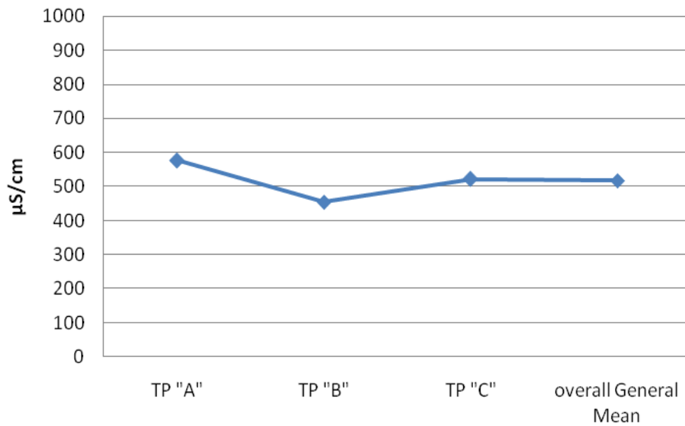
Figure 5: Average values of EC measured for treated grey water
